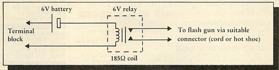
Figure 4. Connection to flash unit
